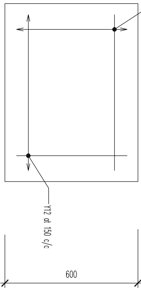
PLAN OF FOOTING
