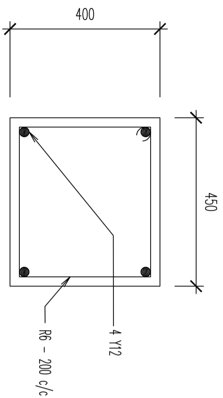
SECTION C - C
